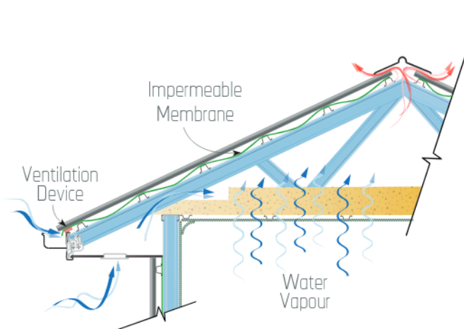
FIG 1(a) Pitched roof with a flat ceiling
