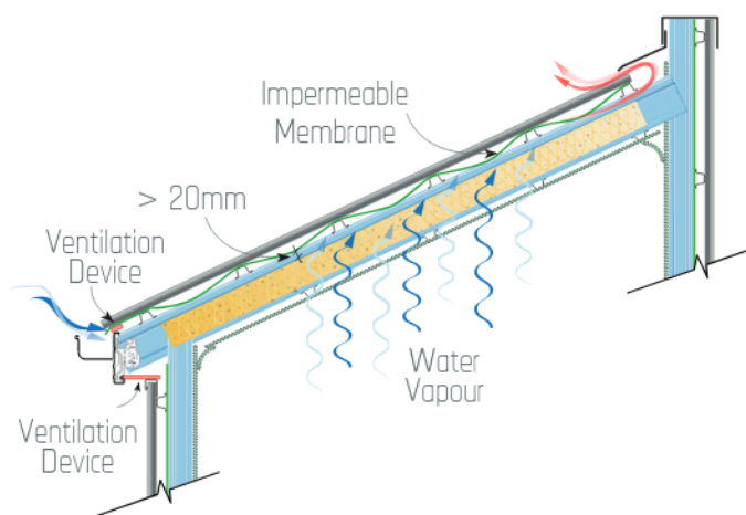
FIG 1(b) Skillion roof
