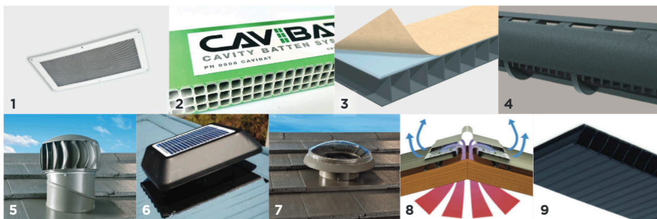
FIG 6 - Examples of vent devices.
