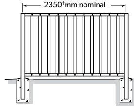
Fence Type SHS3 (3 infill sheets, square hollow section posts, infills screwed to rails)
