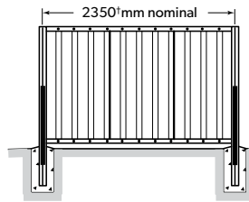
Fence Type FS3 (3 infill sheets, flat post stiffener, infills screwed to rails)
