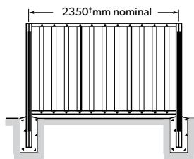
Fence Type CS3 (3 infill sheets, channel post stiffener, infills screwed to rails)
