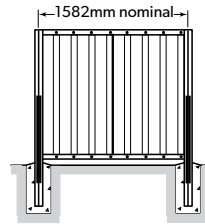
Fence Type FS2 (2 infill sheets, flat post stiffener, infills screwed to rails)
