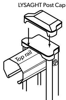
FIGURE 15.2: NEETASCREEN® (& 'PLUS') using universal rail.
