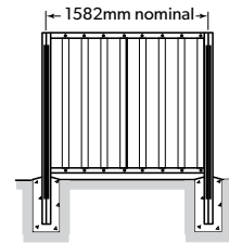
Fence Type CS2 (2 infill sheets, channel post stiffener, infills screwed to rails)
